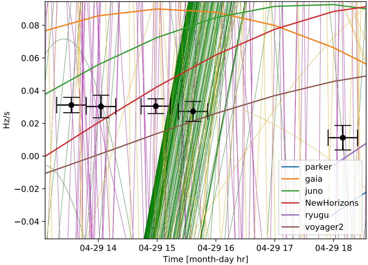
Figure 2. Drift characteristics of non-LEO satellites and deep space probes above the horizon during the event time. The thin green lines are GEO, the magenta are MEO, and the orange are other non-LEO satellites. The thick lines are deep space probes: Parker Solar Probe (blue), Gaia (orange), Juno (green), New Horizons (red), Ryugu (purple) and Voyager 2 (brown). The black data points show the blc1 data, where the x-axis bars are the time of observation and the y-axis bars are 1\sigma error bars. The deep-space probes are closer to the correct order of blc1's drift due to their unique status as near-sidereal sources, but none can explain blc1.
